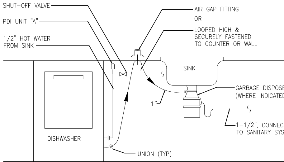
1. RESIDENTIAL DISHWASHER PIPING DETAIL SCALE: NTS
