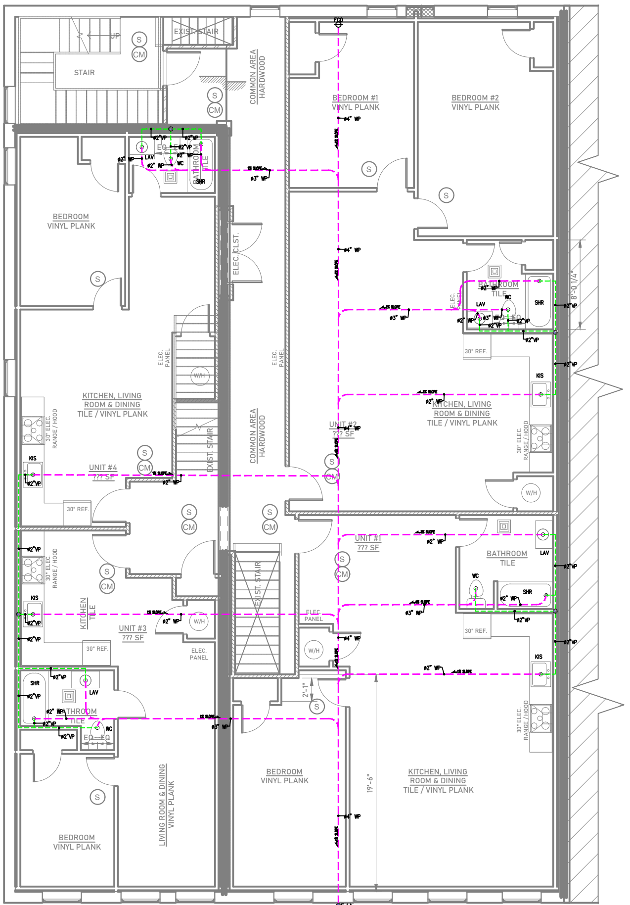
PL 04 SCALE SECOND FLOOR DRAINAGE PLAN 3" = 1'-0"
