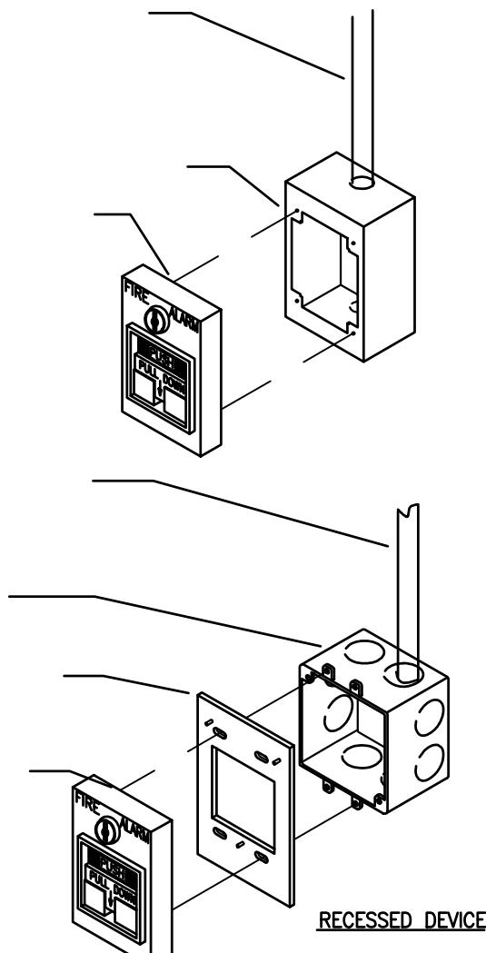
4 TYPICAL MANUAL PULL STATION N.T.S.
