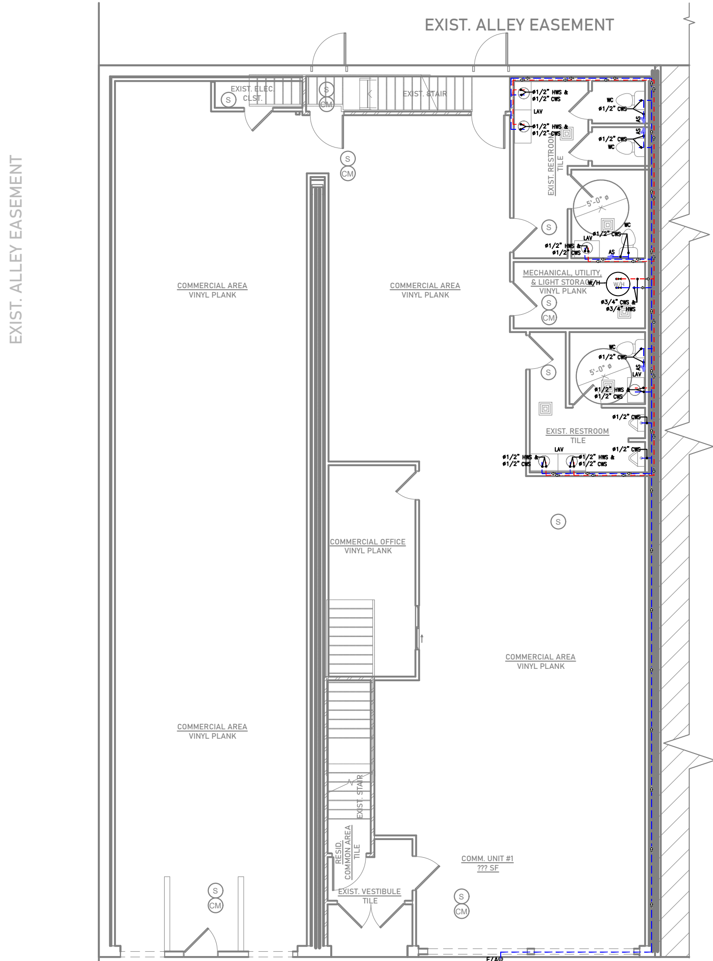
PL 03 FIRST FLOOR WATER SUPPLY PLAN SCALE 3" = 1'-0"
