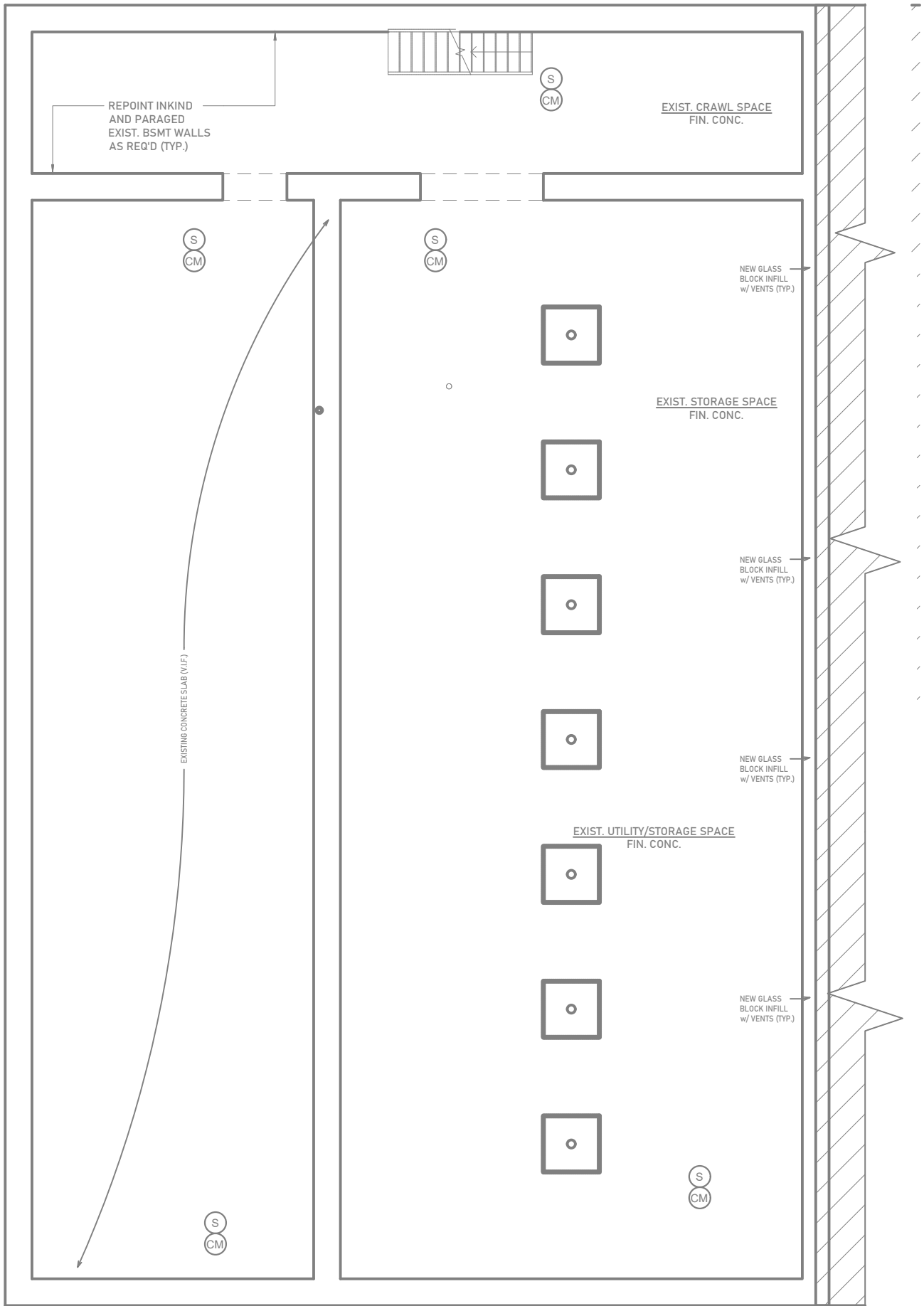
PL 03 BASEMENT FLOOR WATER SUPPLY PLAN SCALE 3" = 1'-0"
