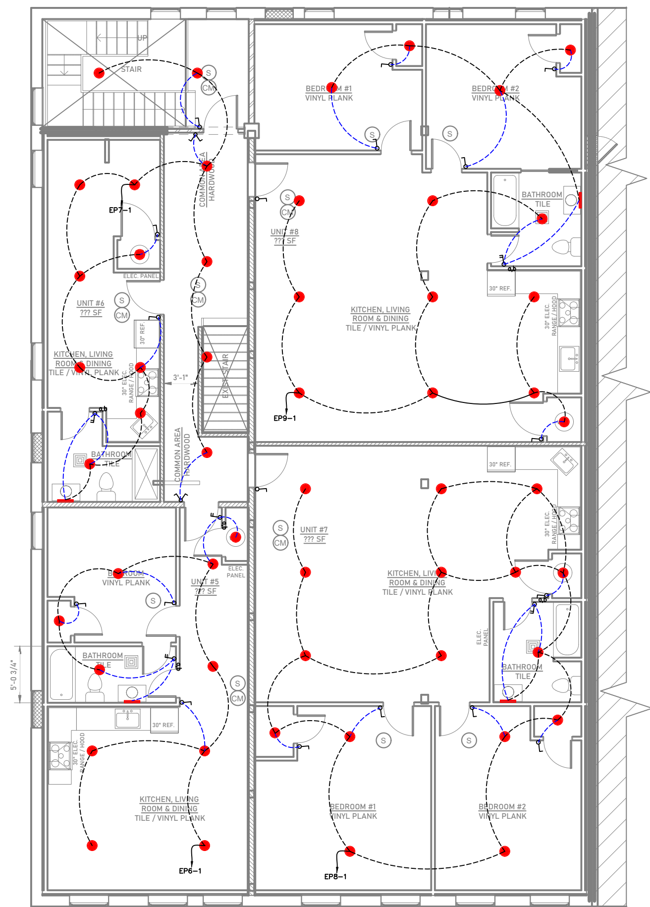
THIRD FLOOR LIGHTING PLAN SCALE 3" = 1'-0"
