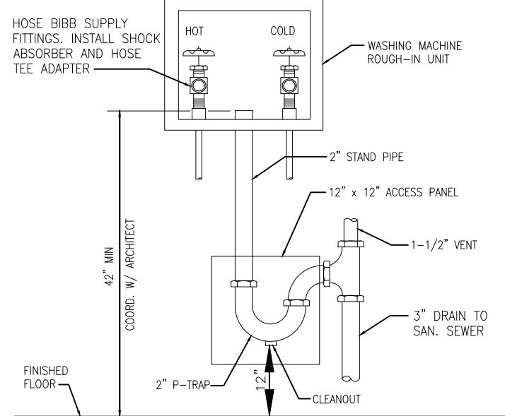
1. RESIDENTIAL WASHING MACHINE CONNECTION DETAIL SCALE: NTS
