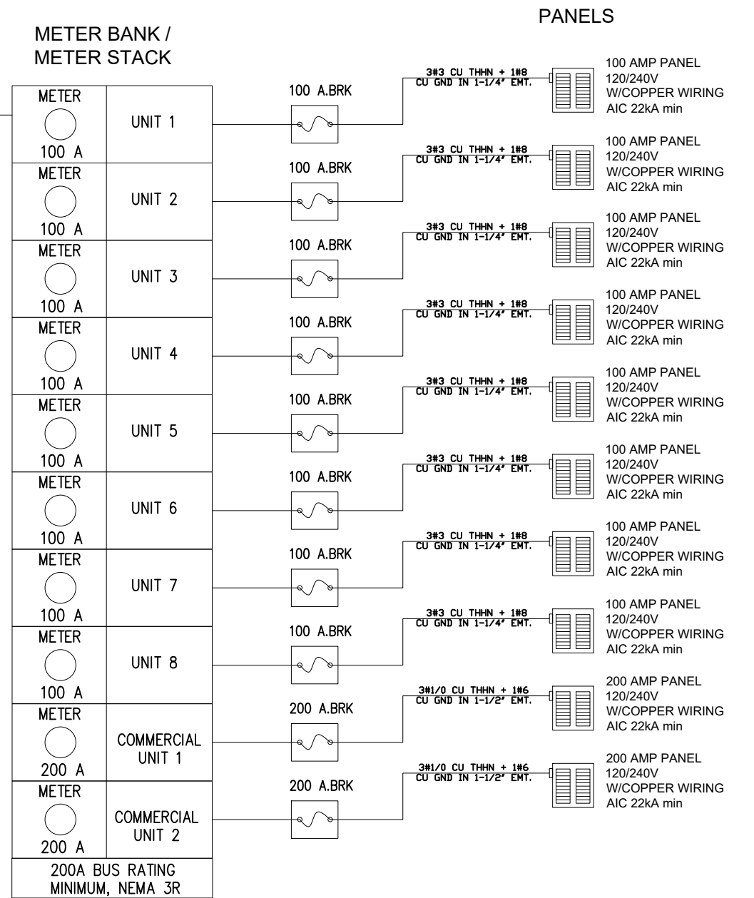
EL 03 / SCALE SINGLE LINE DIAGRAM NTS
