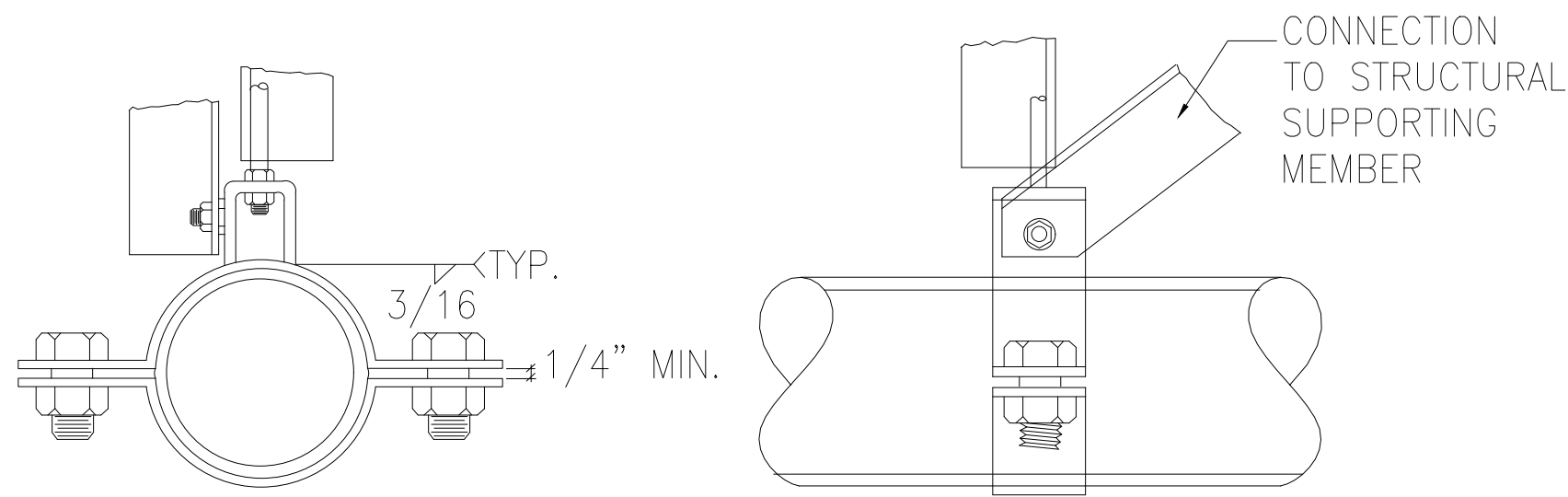
1. TYPICAL LONGITUDINAL PIPE BRACING SCALE: NTS
