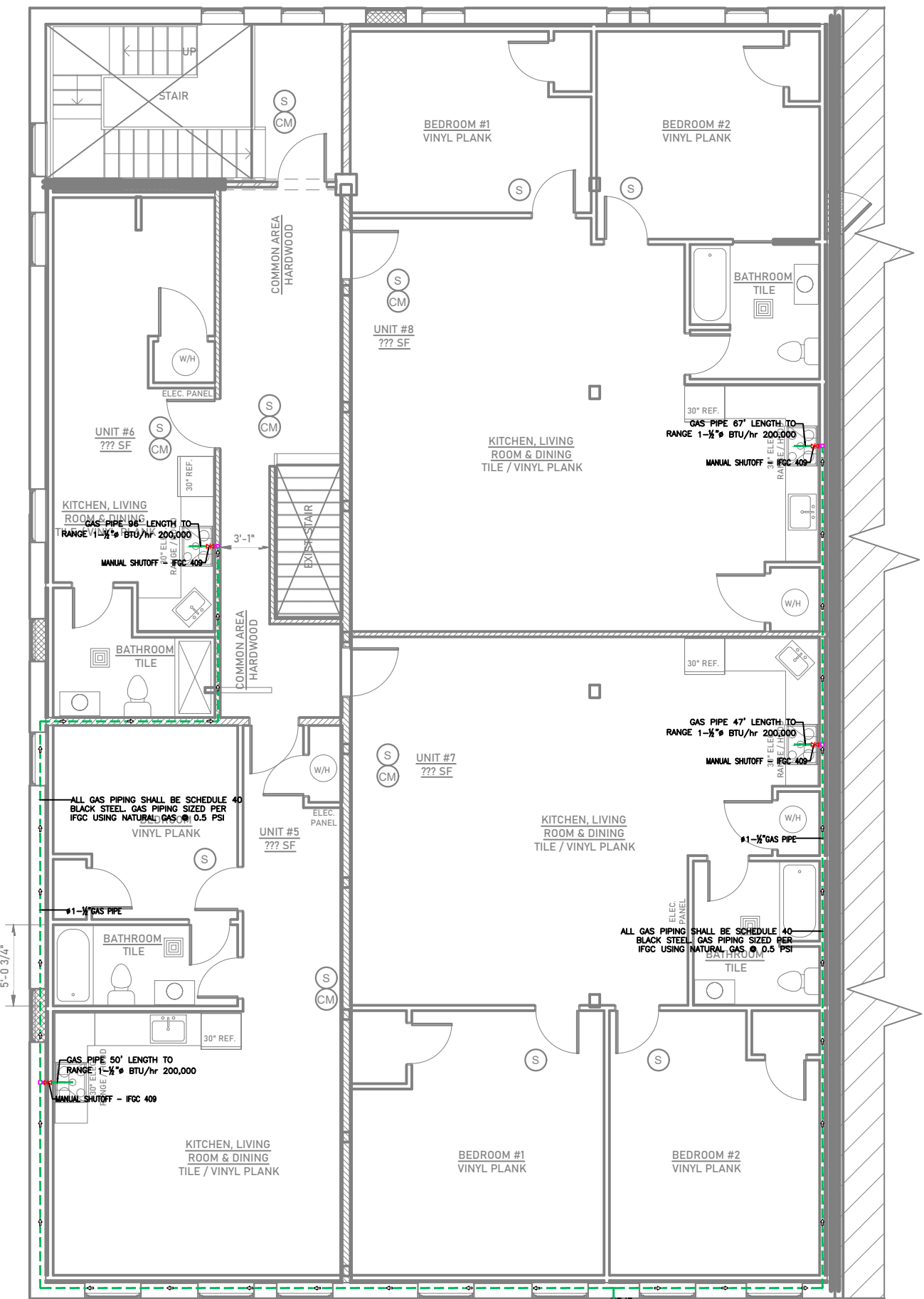
PL 07 SCALE THIRD FLOOR GAS SUPPLY PLAN 3" = 1'-0"
