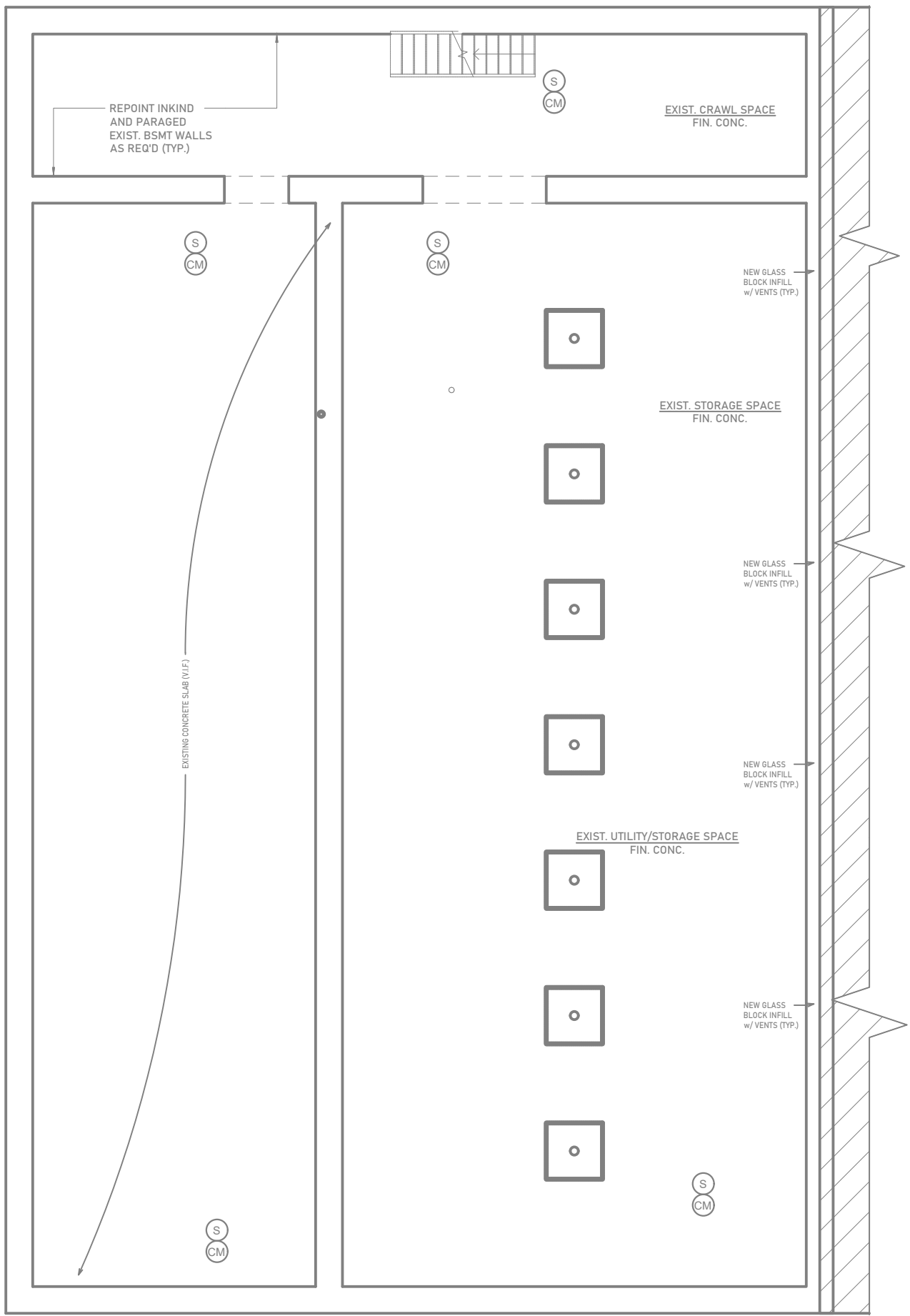
PL 02 SCALE BASEMENT FLOOR DRAINAGE PLAN 3" = 1'-0"
