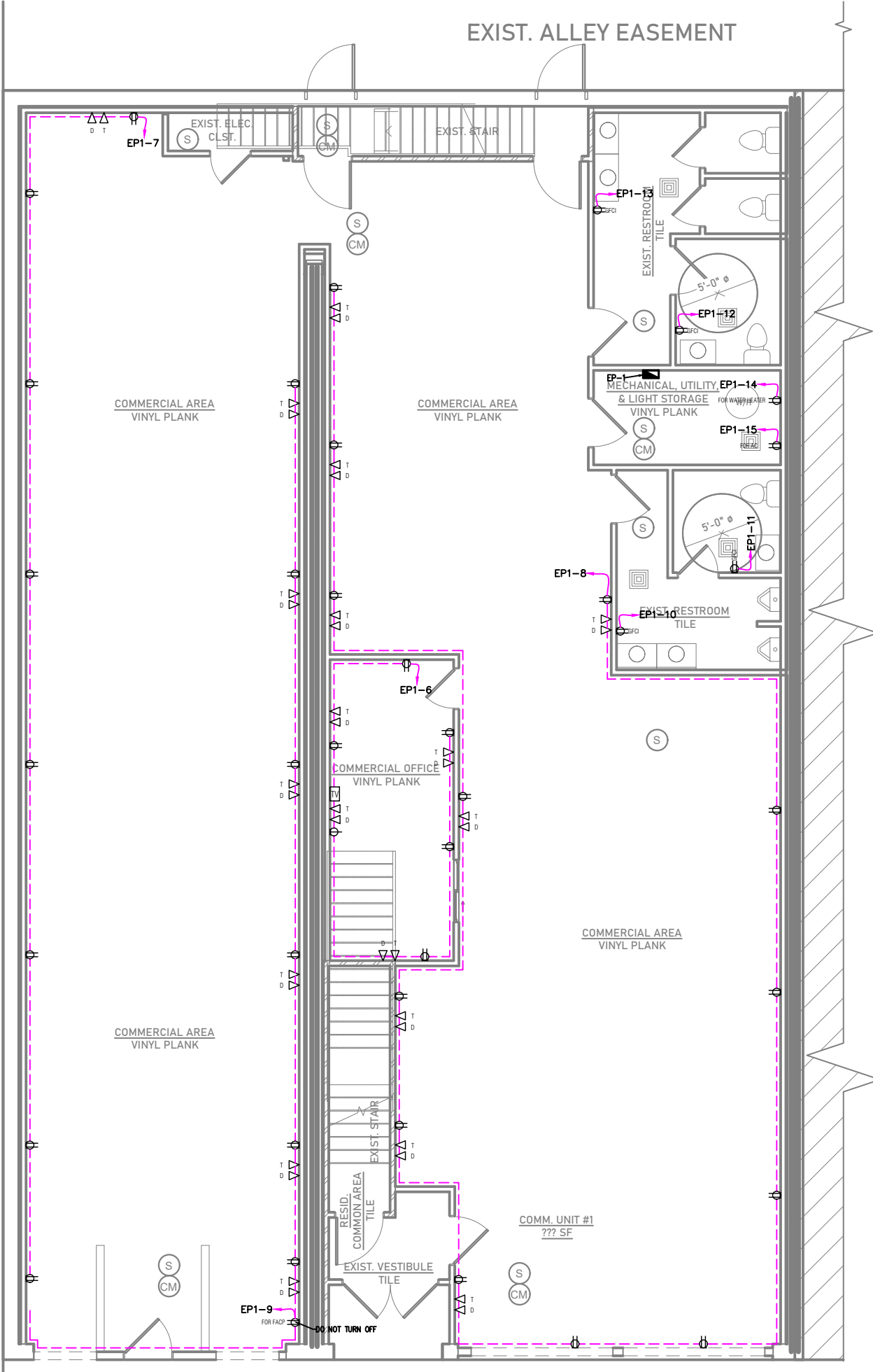
EL 83 / SCALE FIRST FLOOR POWER PLAN 3" = 1'-0"
