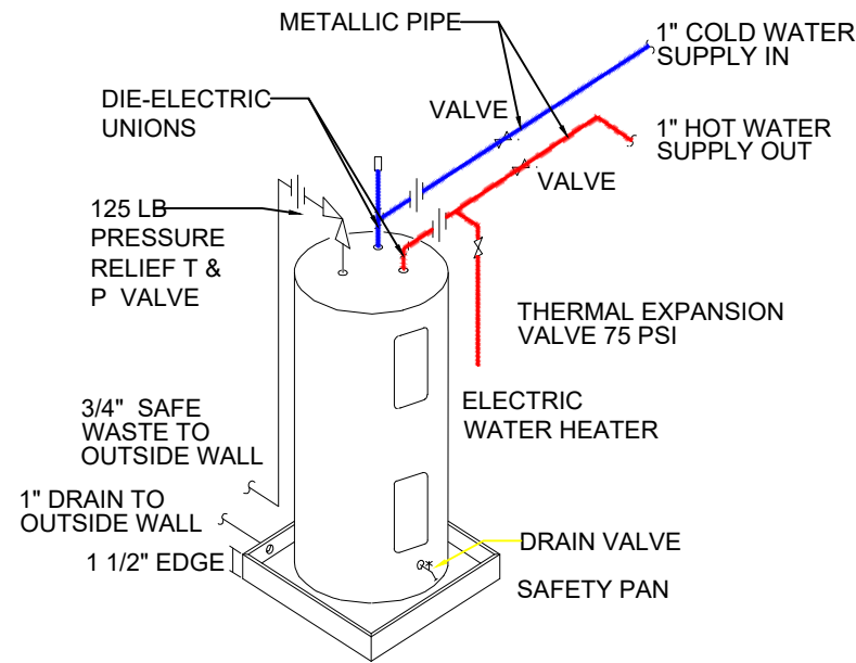
1. WATER HEATER INSTALLATION DETAILS SCALE: NTS
