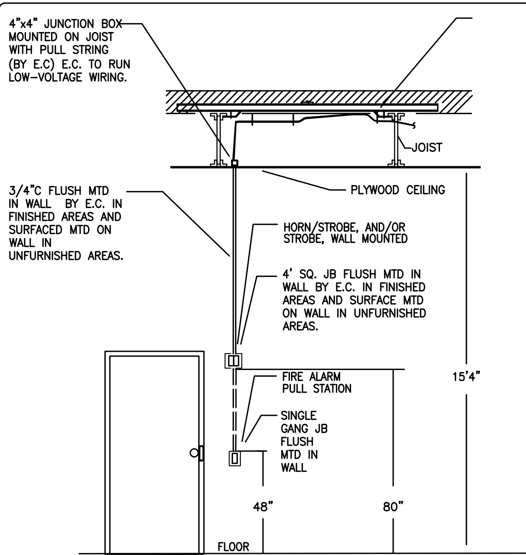
1 MANUAL PULL STATION AND SIGNAL MOUNTING. N.T.S.
