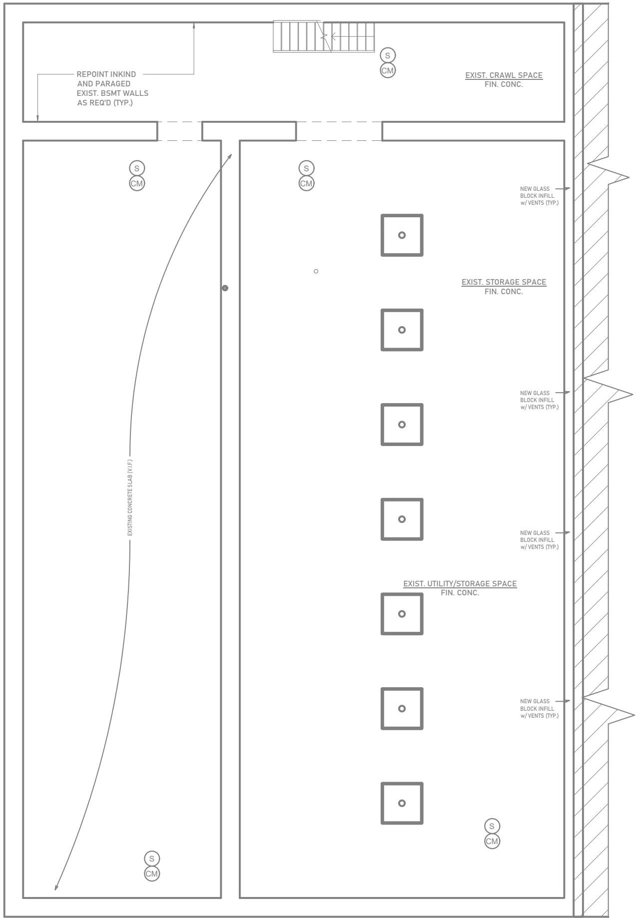
EL 82 / SCALE BASEMENT FLOOR POWER PLAN 3" = 1'-0"
