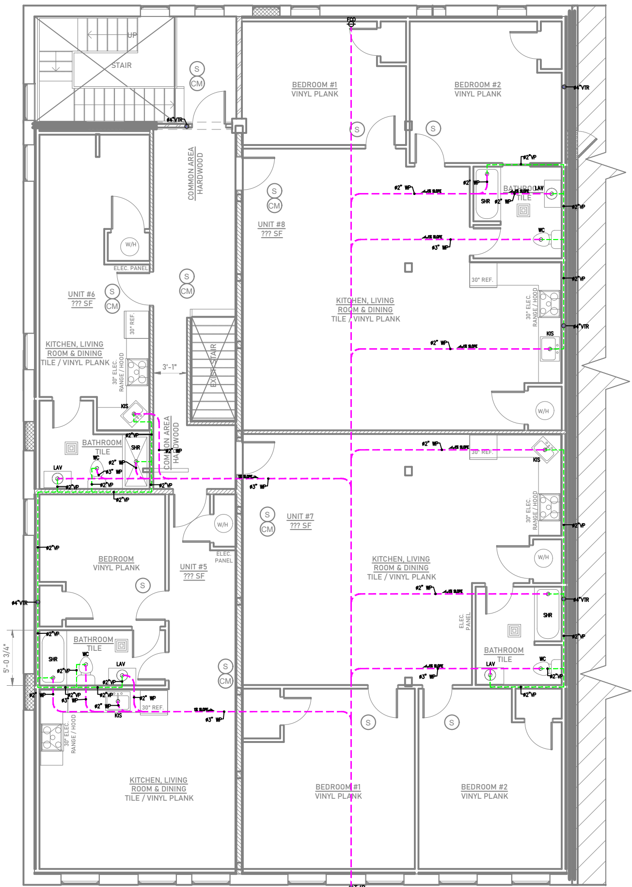
PL 05 SCALE THIRD FLOOR DRAINAGE PLAN 3" = 1'-0"
