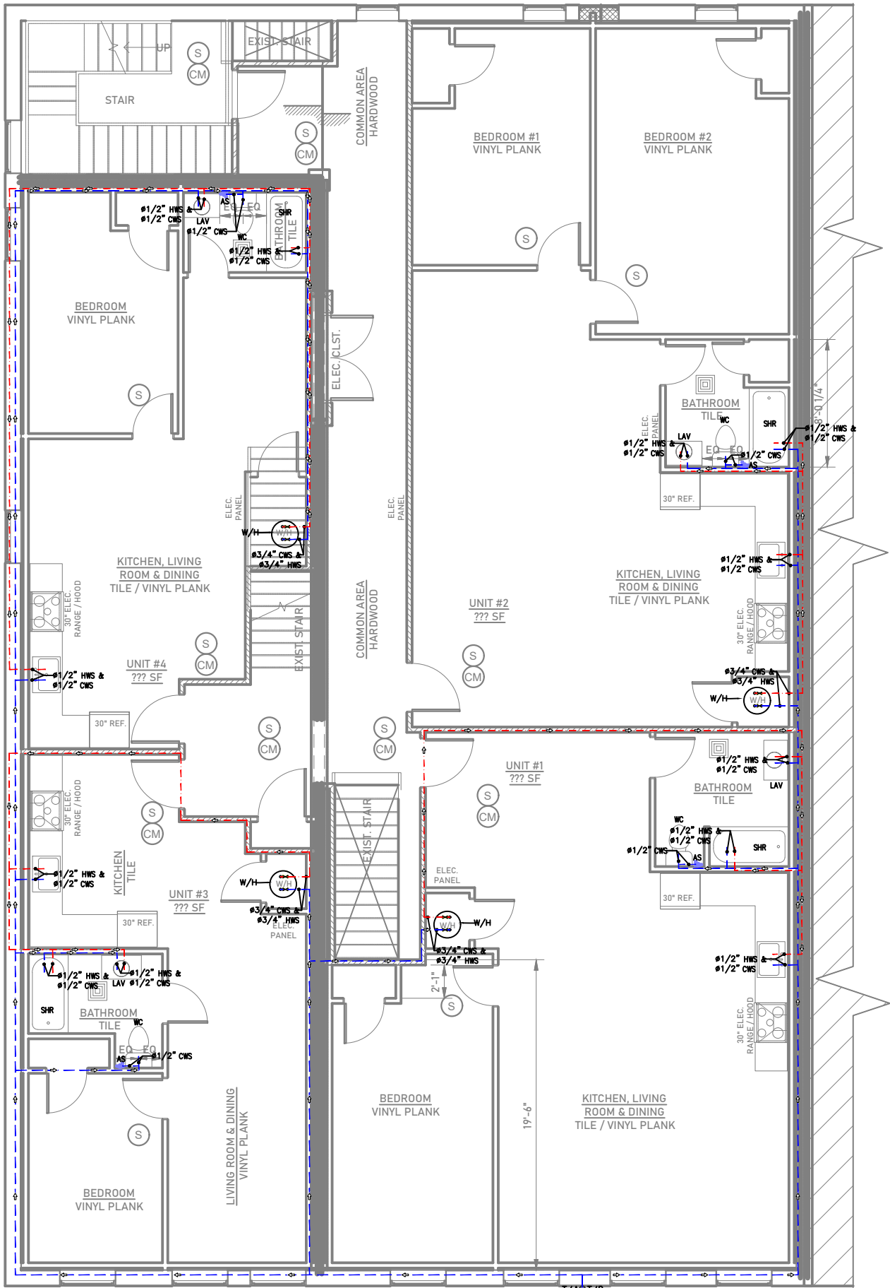
PL 03 SECOND FLOOR WATER SUPPLY PLAN SCALE 3" = 1'-0"
