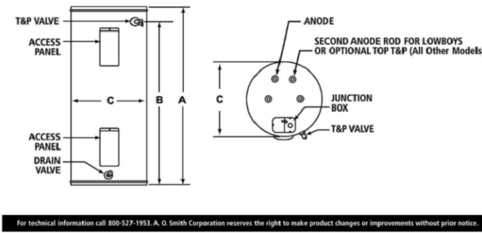
1. WATER HEATER INSTALLATION DETAILS SCALE: NTS
