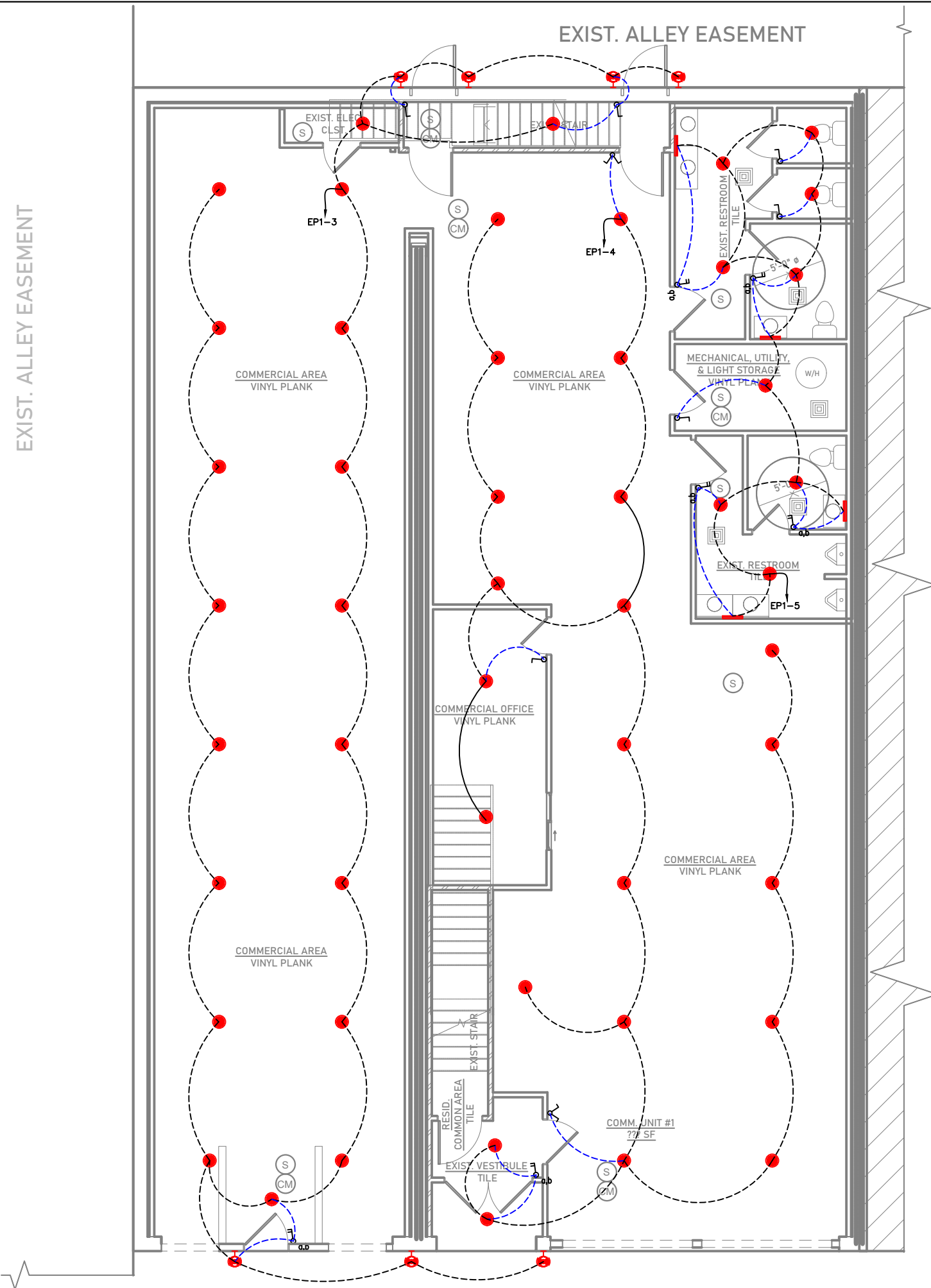
FIRST FLOOR LIGHTING PLAN SCALE 3" = 1'-0"
