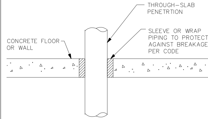
1. PIPE SLAB PENETRATION SCALE: NTS
