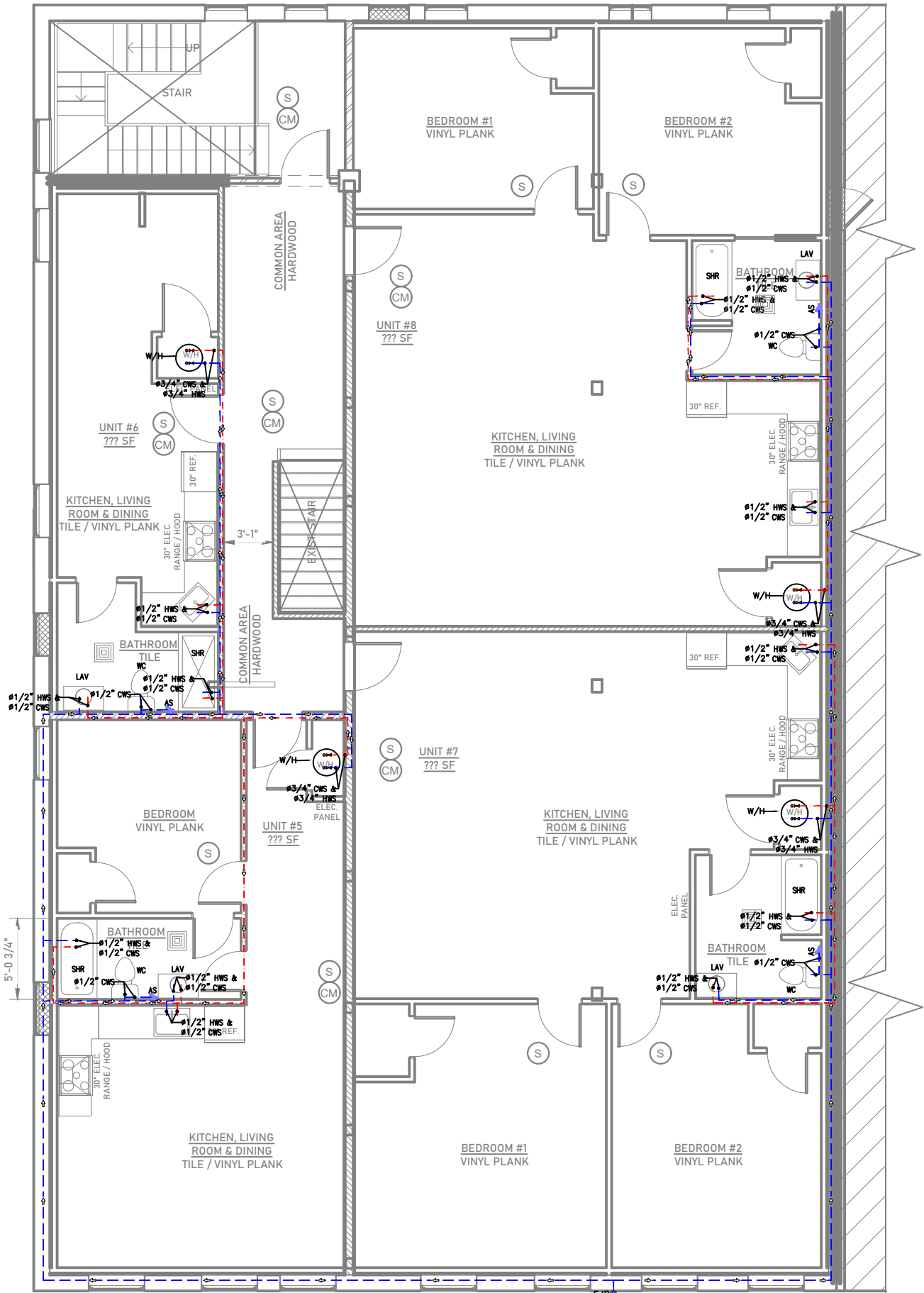
PL 03 THIRD FLOOR WATER SUPPLY PLAN SCALE 3" = 1'-0"
