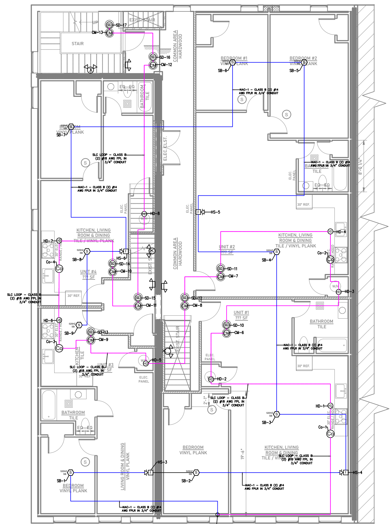
FA 01 SECOND FLOOR FIRE ALARM PLAN 3" = 1'-0"
