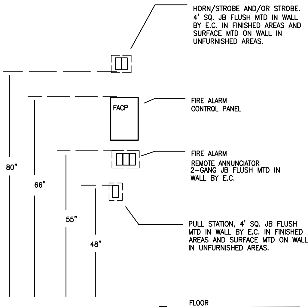
5 DEVICE MOUNTING HEIGHT DETAILS N.T.S.
