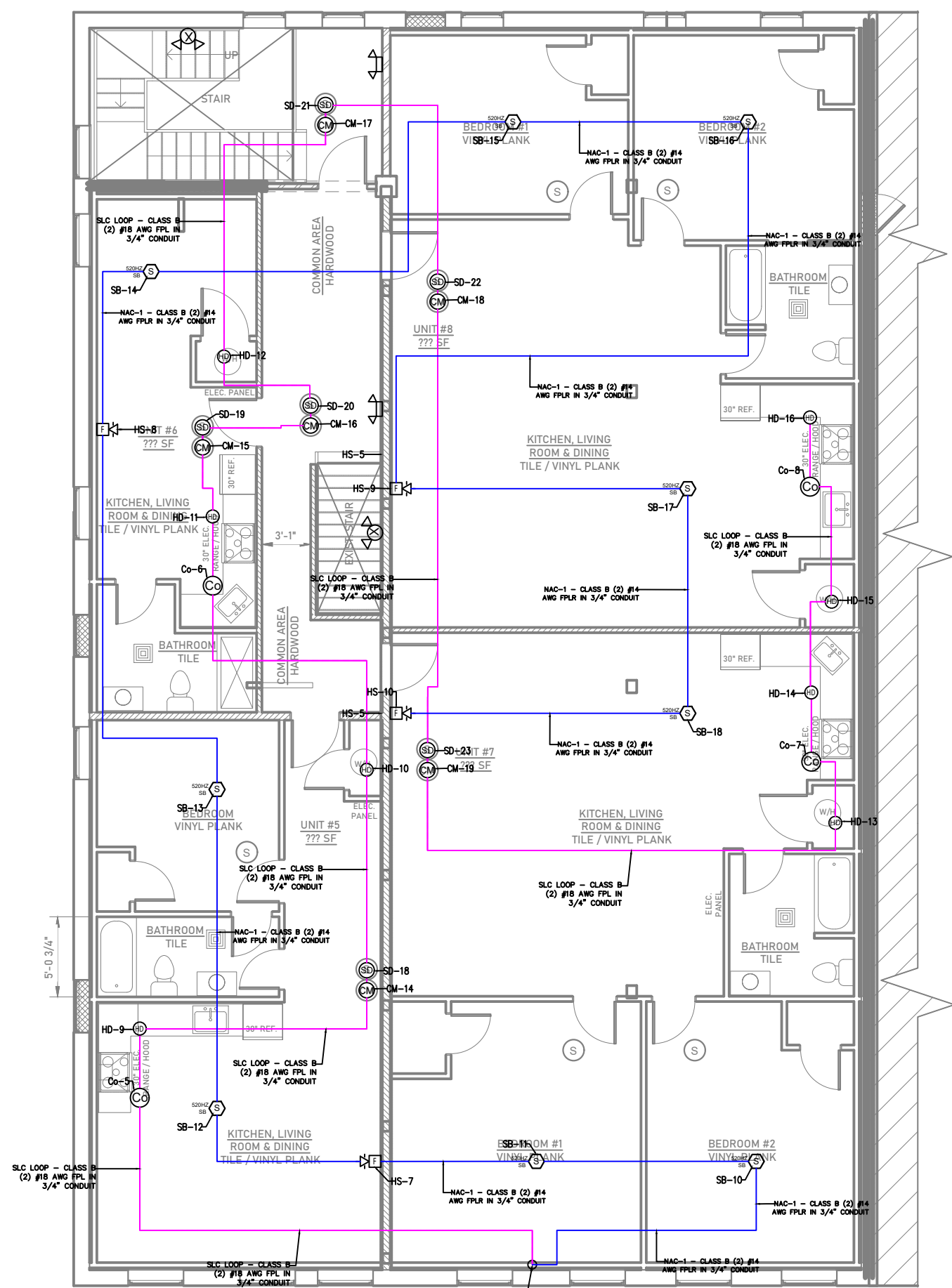
FA 01 THIRD FLOOR FIRE ALARM PLAN 3" = 1'-0"
