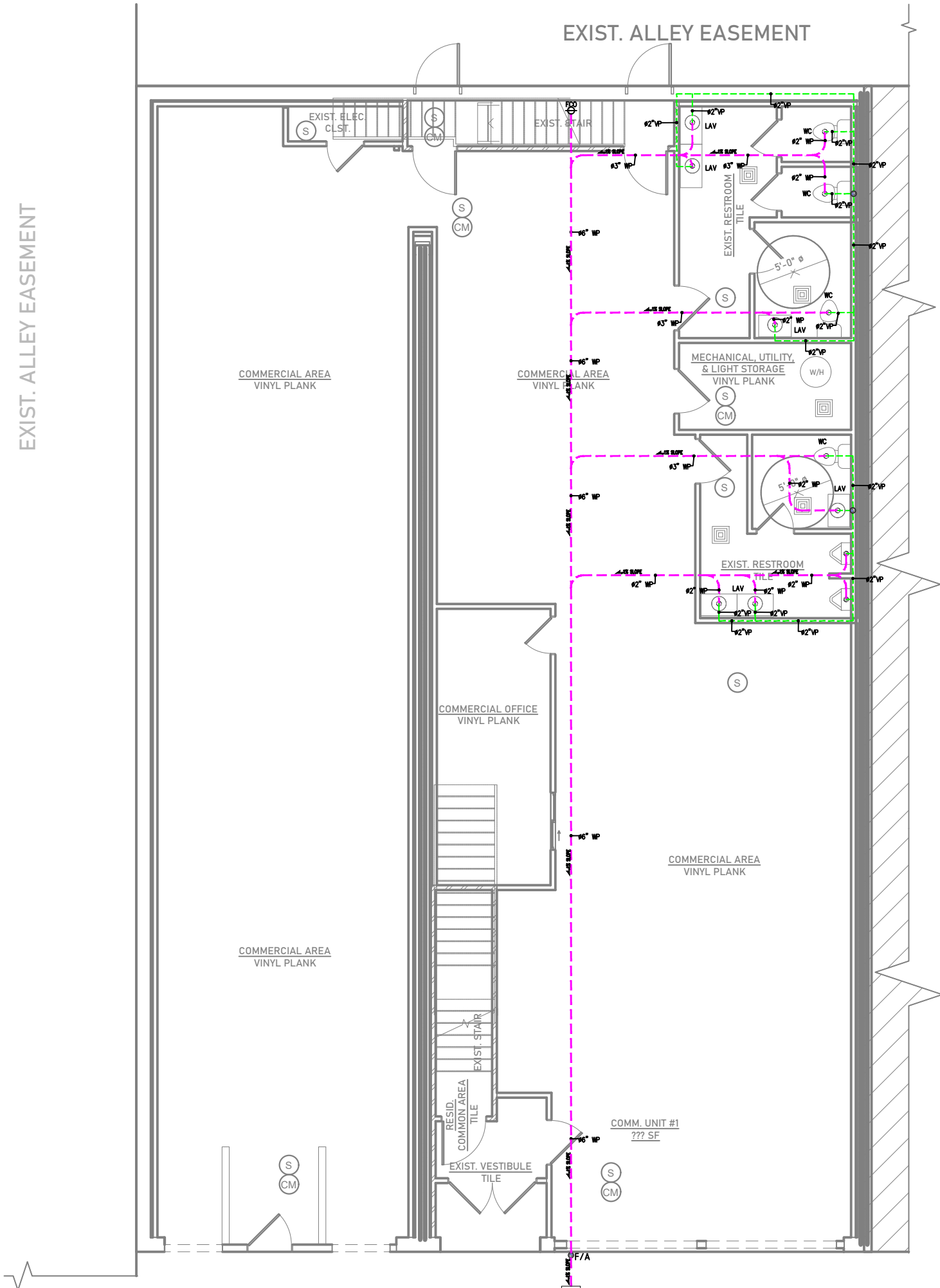
PL 03 SCALE FIRST FLOOR DRAINAGE PLAN 3" = 1'-0"
