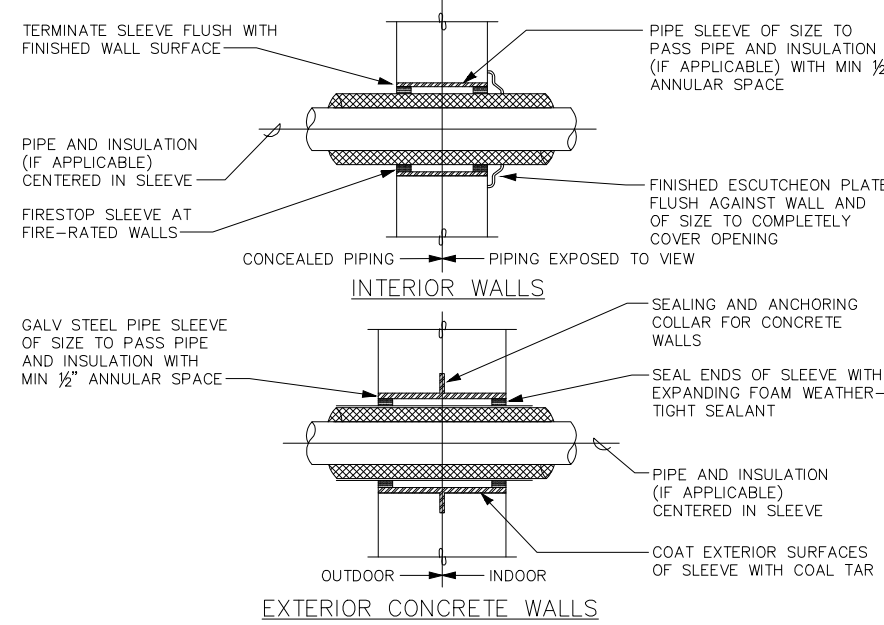
1. PIPE SLEEVES THROUGH WALLS SCALE: NTS
