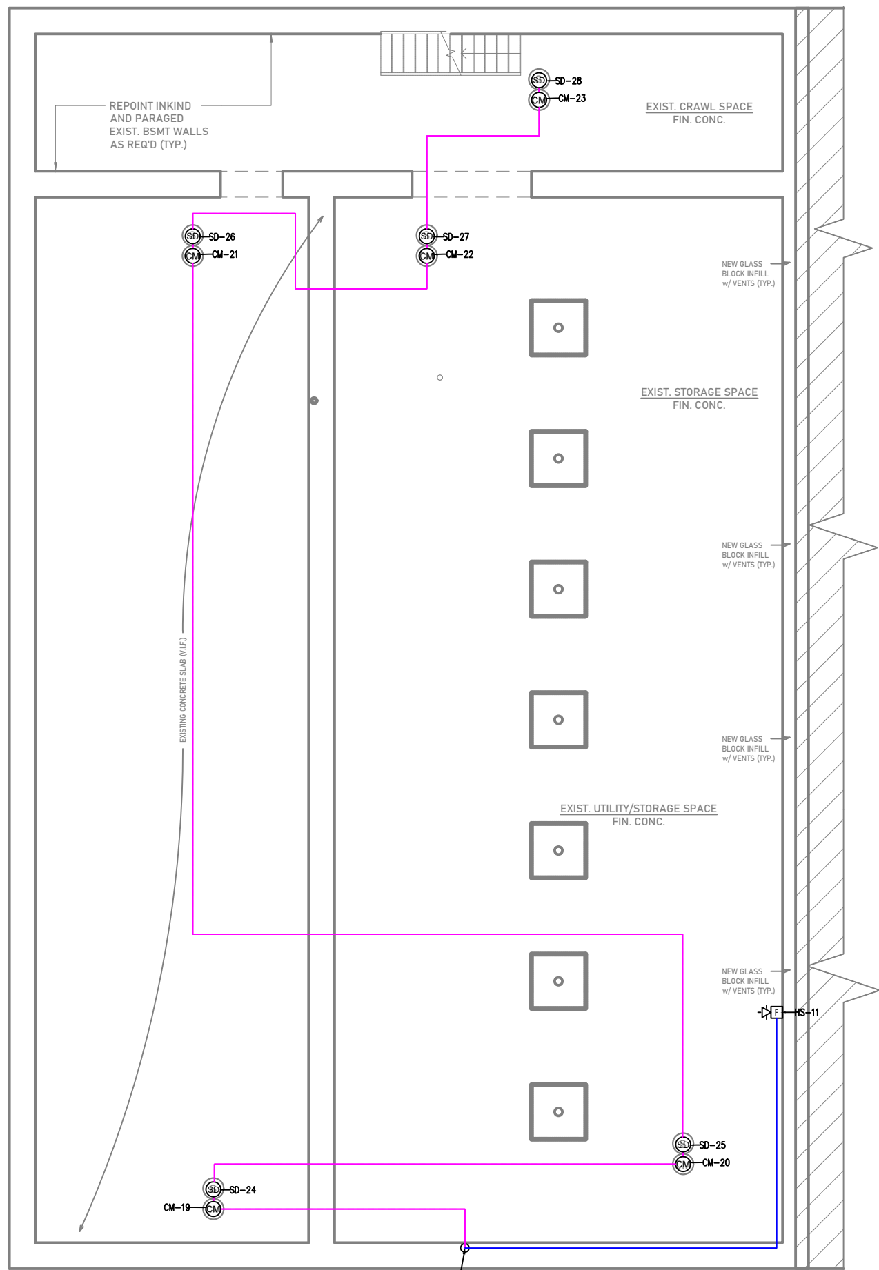
FA 01 BASEMENT FLOOR FIRE ALARM PLAN 3" = 1'-0"
