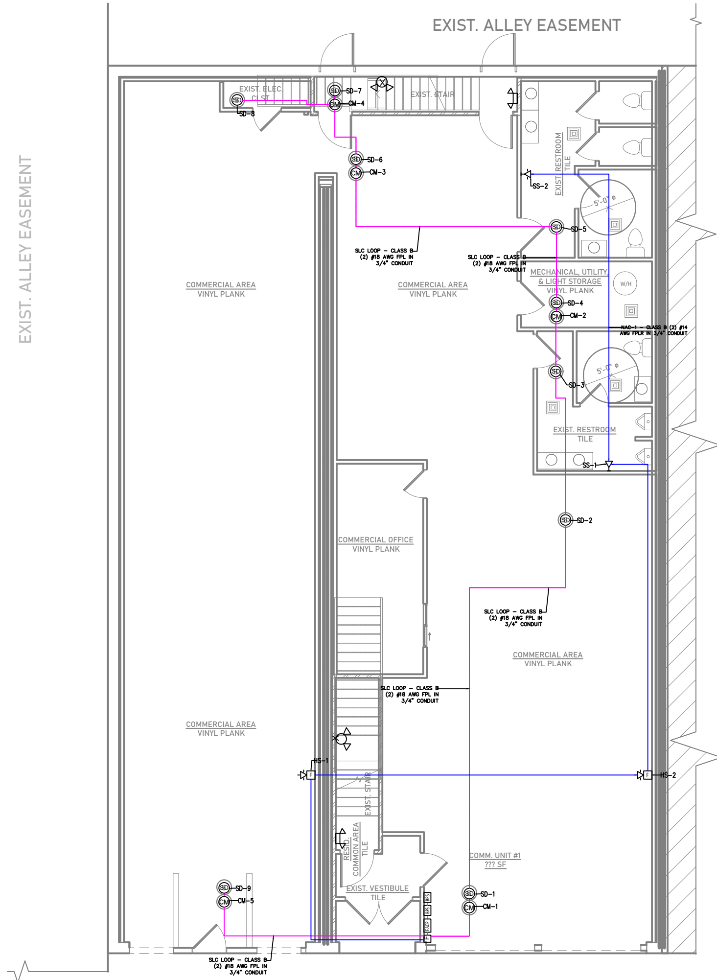
FA 01 FIRST FLOOR FIRE ALARM PLAN 3" = 1'-0"
