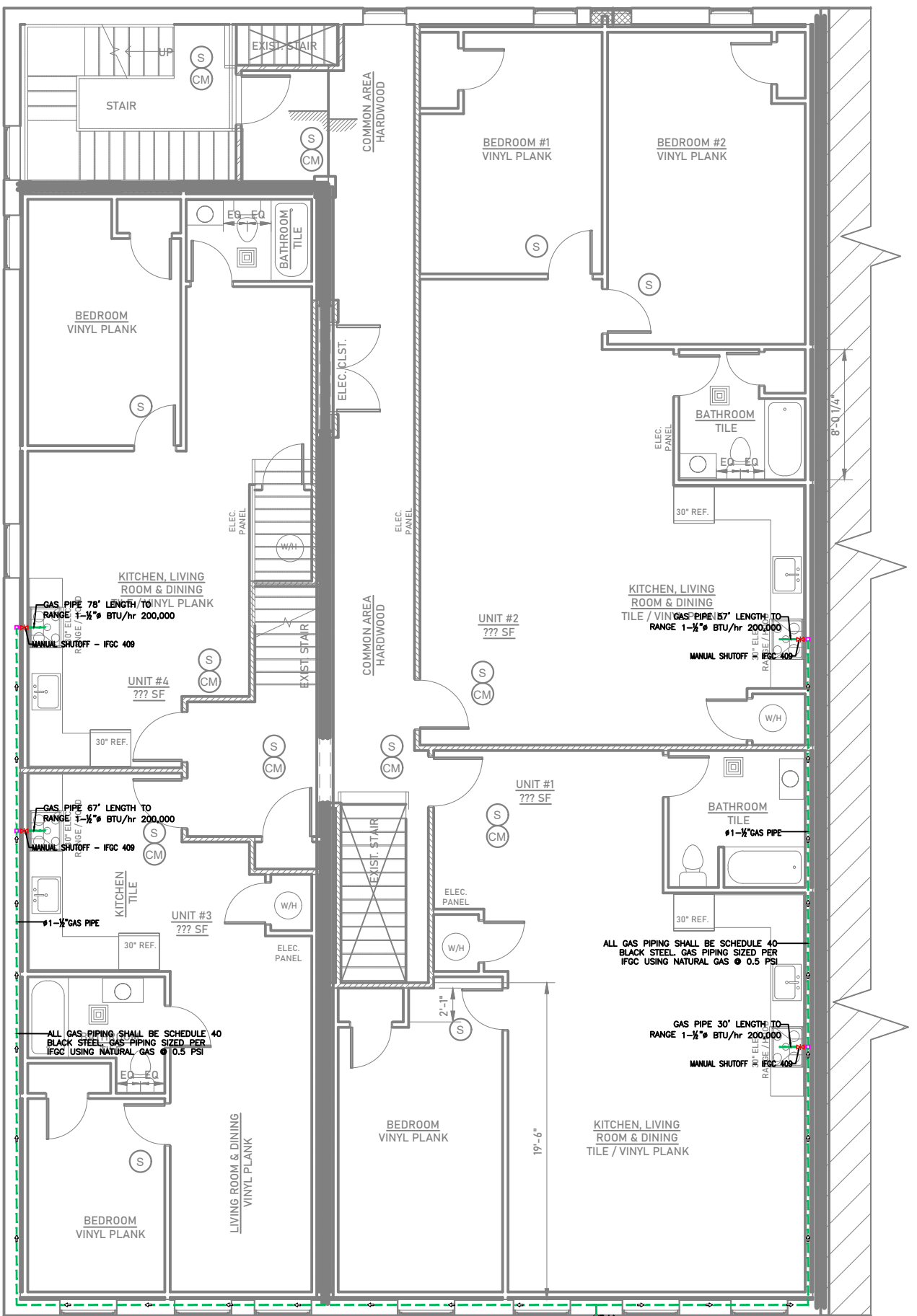
PL 07 SCALE SECOND FLOOR GAS SUPPLY PLAN 3" = 1'-0"
