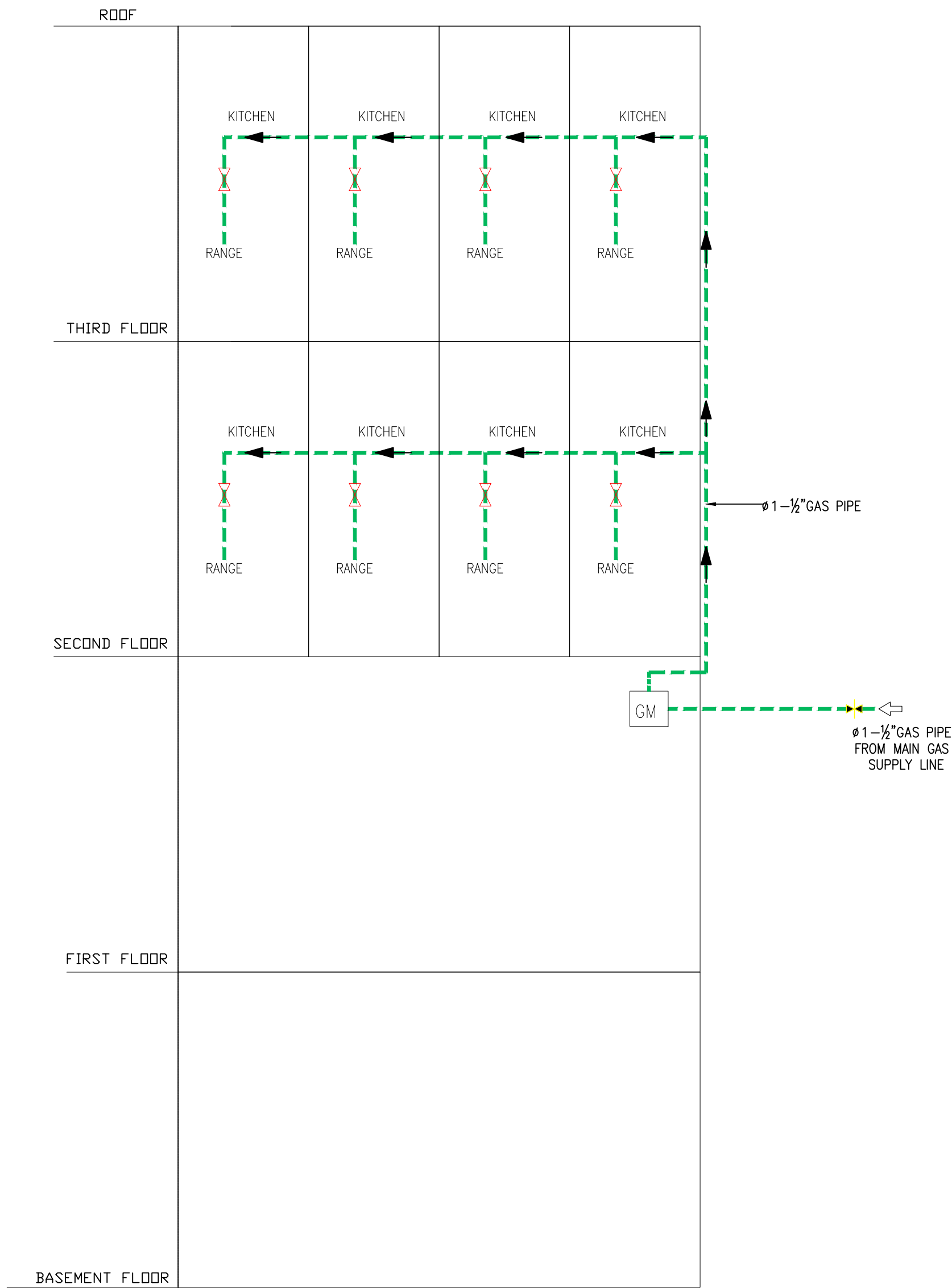
PL 07 SCALE GAS SUPPLY SYSTEM RISER DIAGRAM NTS
